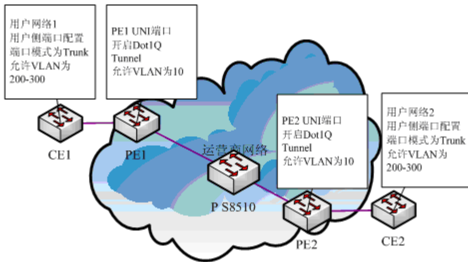
Figure 3 Typical configuration of Dot1Q tunnel
